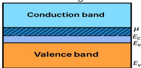
Figure 1. Energy diagram of a degenerate n -type semiconductor; \mu - E_c represents the electron-filled portion of the conduction band.
